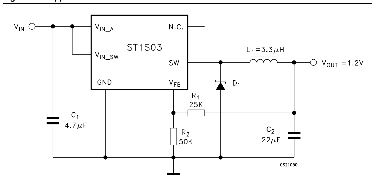
Figure 3. Application circuits
