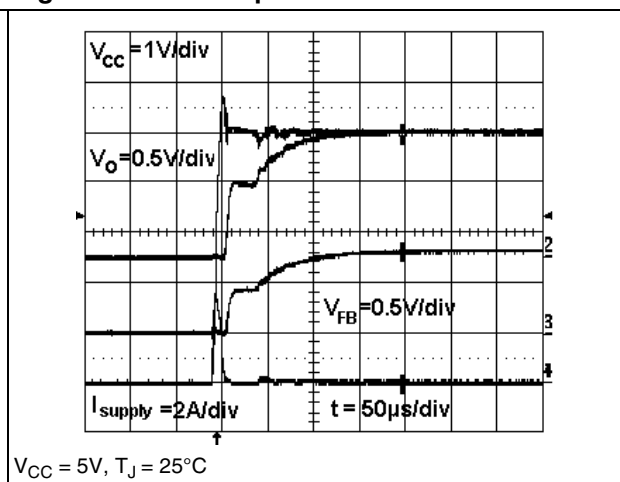
Figure 21. Start-Up transient
