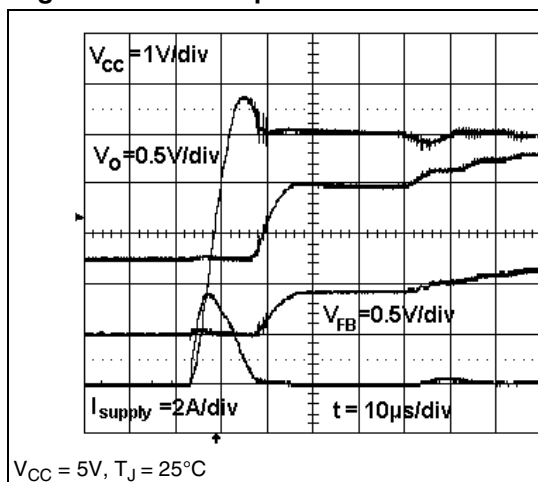
Figure 20. Start-Up transient
